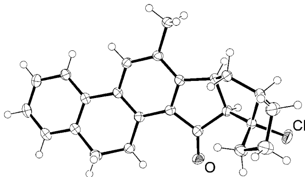
Figure 1. Structure of the hexacycle 17 in the crystal. [19]
