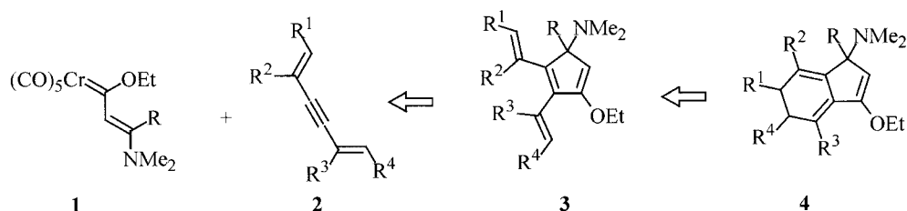
Scheme 1. Conceived synthesis of 1,2-dialkenyl-5-dimethylamino-3-ethoxycyclopentadienes 3 and their 6\pi -electrocyclization to six-ring annulated protected cyclopentenones 4 .
