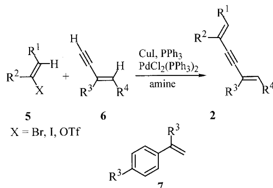
Scheme 2. Synthesis of various 1,5-dien-3-ynes 2 . For details see Table 1.
