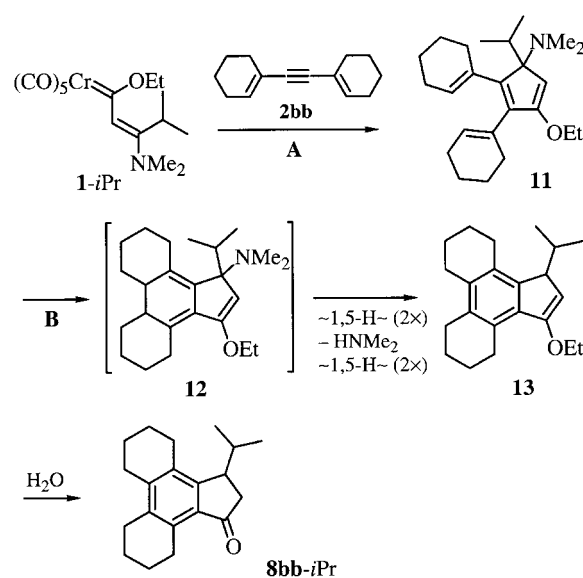
Scheme 4. Mechanistic rationalization of the formation of indanone derivatives of type 8bb-iPr . A: formal [3+2] cycloaddition. B: 6 \pi -electrocyclization.
