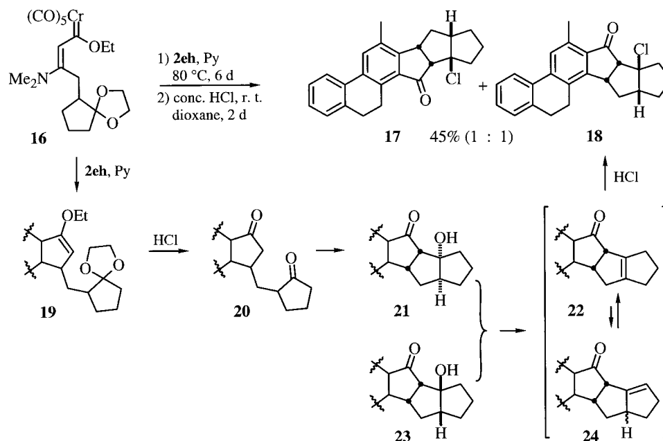
Scheme 6. Access to hexacycles 17/18 in a one-pot operation from complex 16 and diyne 2eh . The mechanistic details are shown for one of the two regioisomers only.
