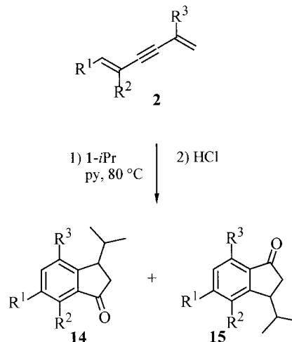
Scheme 5. Synthesis of tetracyclic compounds 14/15 with steroid-like skeletons via complex 1- i Pr and 1,5-dien-3-yne 2 . For details see Table 3.
