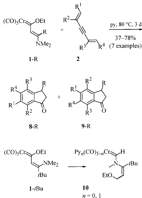
Scheme 3. Synthesis of indenone derivatives 8-R and 9-R . For details see Table 2.
